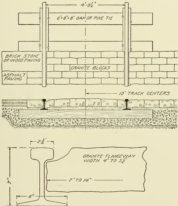
Fig. 221. Plan and Section of Typical City Track
